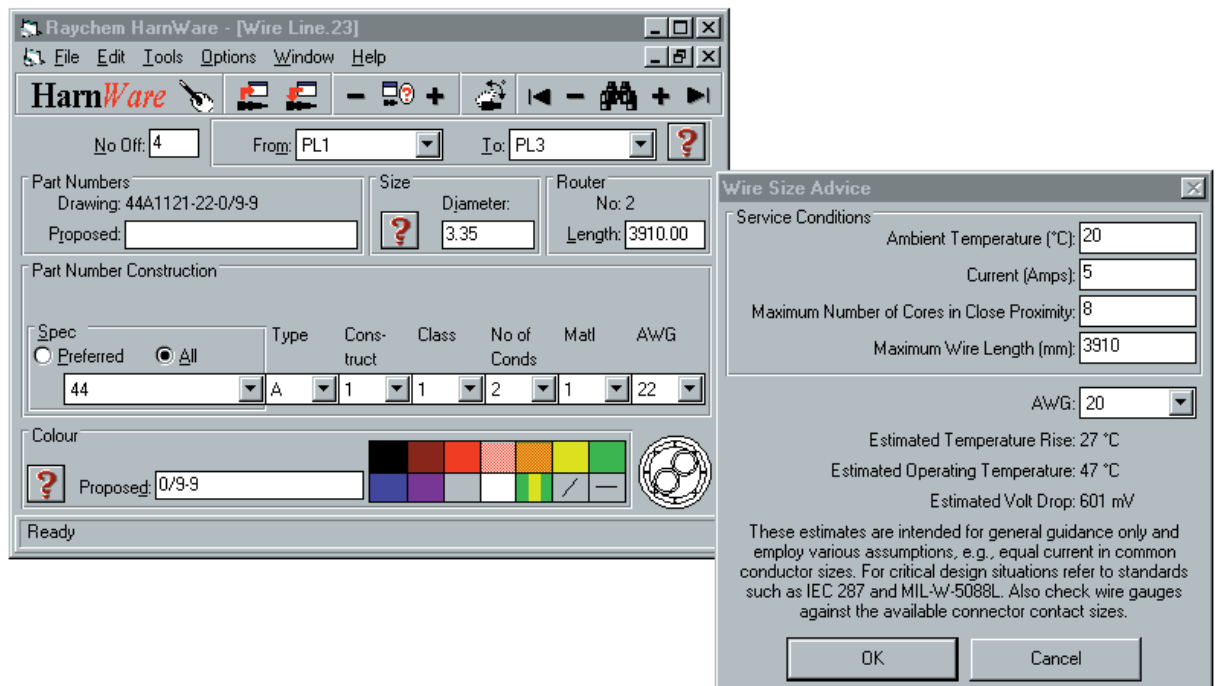
Fig. 4 Guidance on choosing wire type and wire gauge
